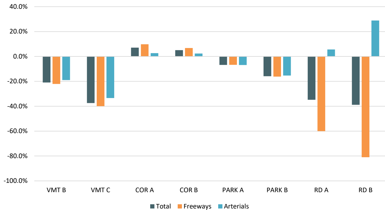
Figure 29 Percent Change in Vehicle Hours of Delay – Region (2-Hour PM Peak)
